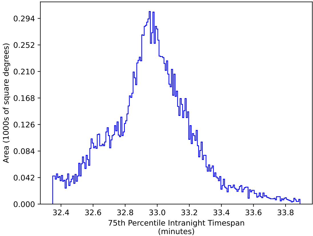
extra_ss_neo3_v3.4_10yrs WFD y band: 75th Percentile Intranight Timespan
