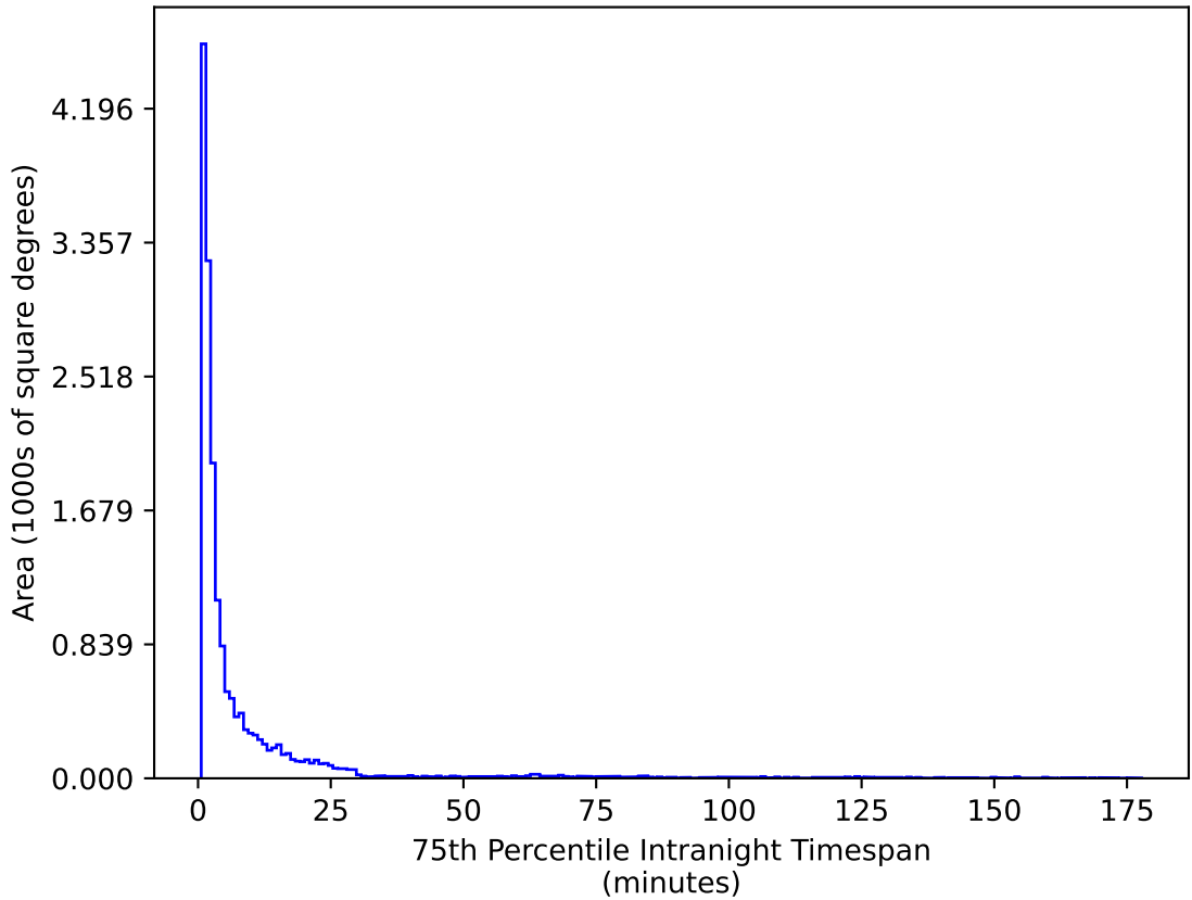
extra_ss_neo3_v3.4_10yrs WFD u band: 75th Percentile Intranight Timespan
