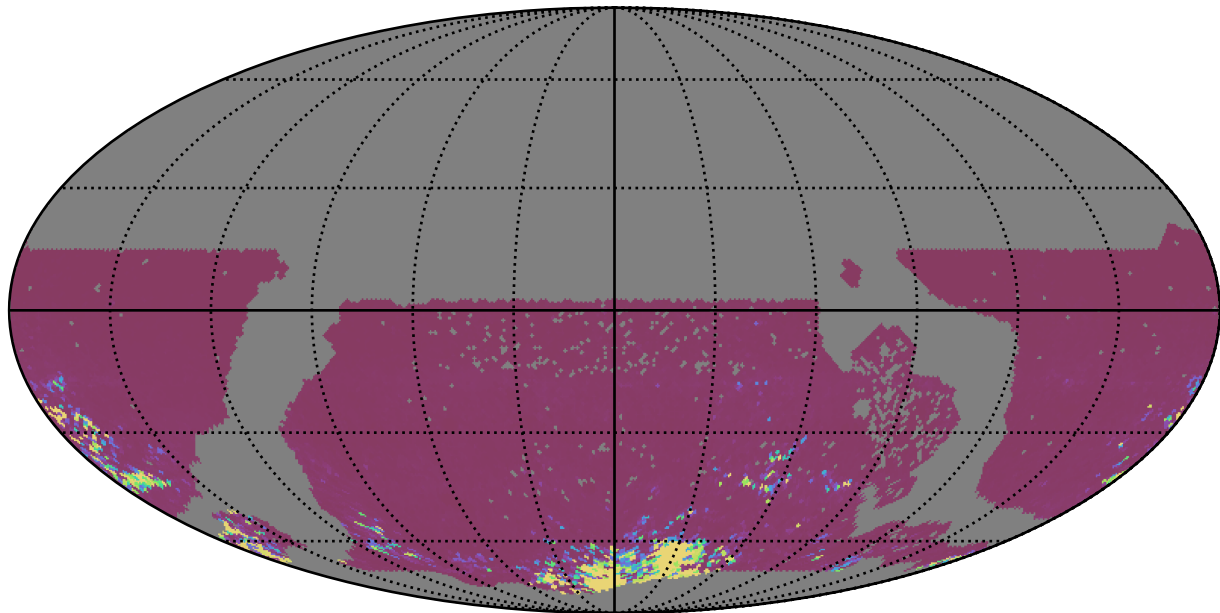
extra_ss_neo3_v3.4_10yrs WFD ri bands: 75th Percentile Intranight Timespan
