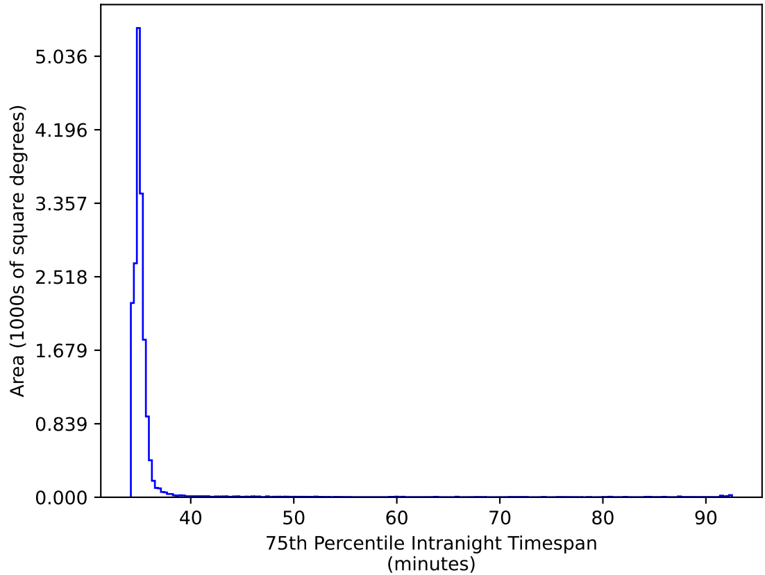
extra_ss_neo3_v3.4_10yrs WFD ri bands: 75th Percentile Intranight Timespan
