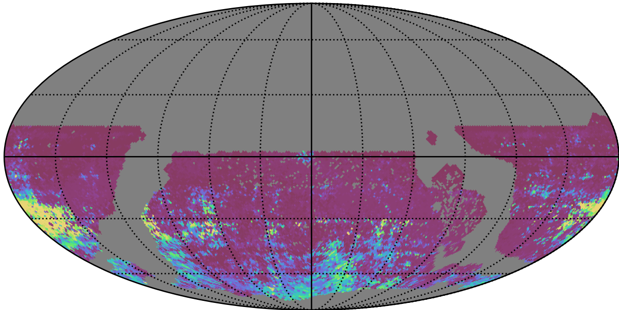
extra_ss_neo3_v3.4_10yrs WFD r band: 75th Percentile Intranight Timespan
