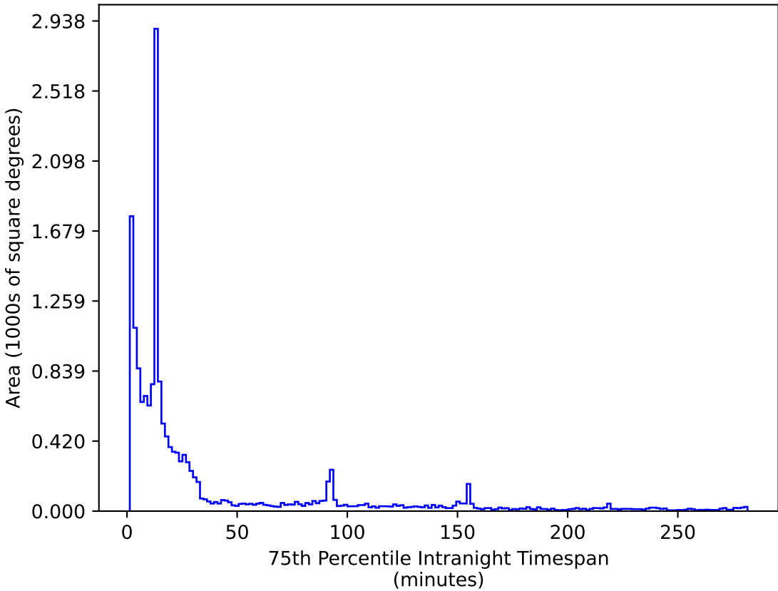
extra_ss_neo3_v3.4_10yrs WFD r band: 75th Percentile Intranight Timespan
