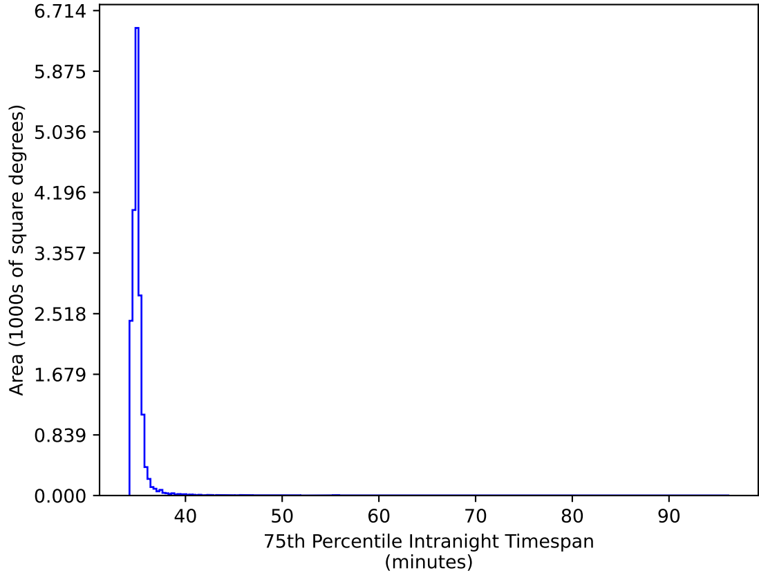
extra_ss_neo3_v3.4_10yrs WFD gr bands: 75th Percentile Intranight Timespan
