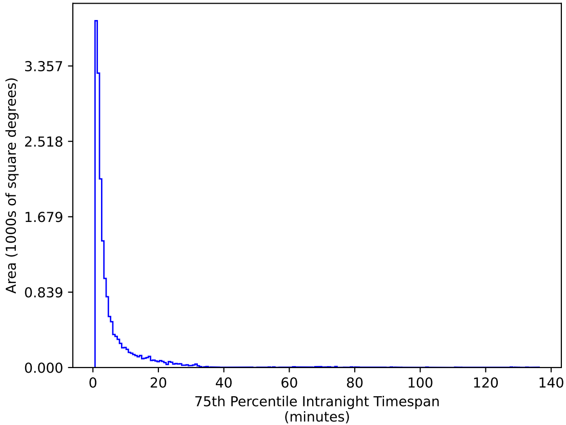
extra_ss_neo3_v3.4_10yrs WFD g band: 75th Percentile Intranight Timespan
