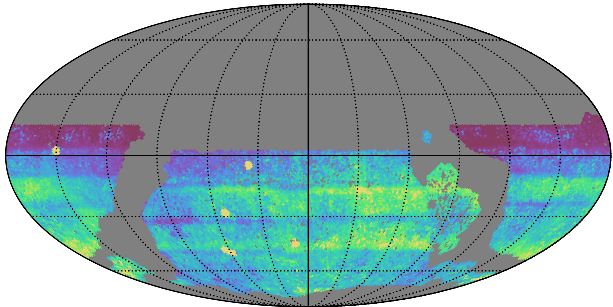
extra_ss_neo3_v3.4_10yrs WFD all bands: 75th Percentile Intranight Timespan
