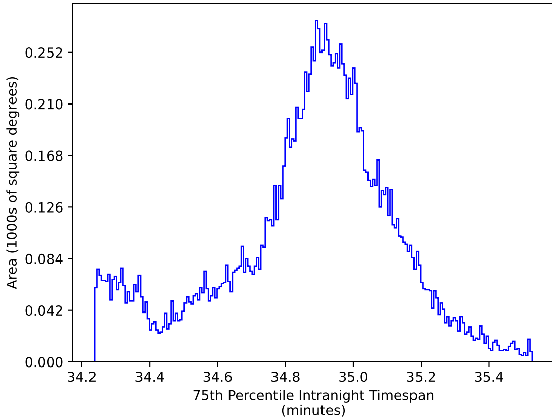
extra_ss_neo3_v3.4_10yrs WFD all bands: 75th Percentile Intranight Timespan
