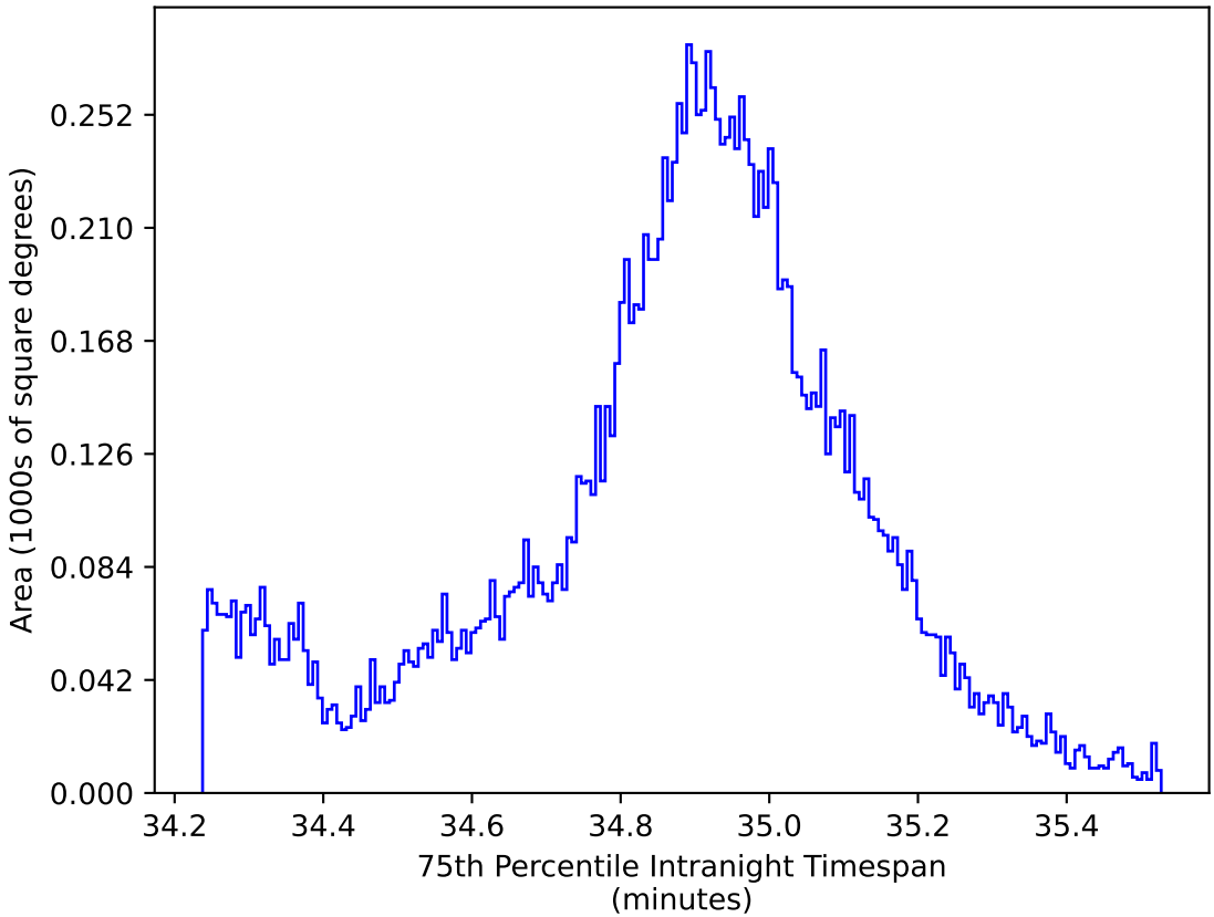
extra_ss_neo3_v3.4_10yrs WFD: 75th Percentile Intranight Timespan
