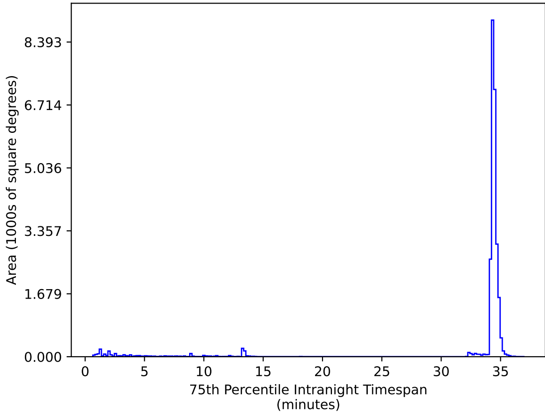
extra_ss_neo3_v3.4_10yrs All sky zy bands: 75th Percentile Intranight Timespan
