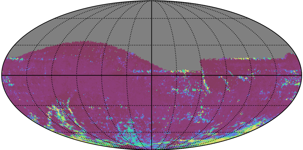
extra_ss_neo3_v3.4_10yrs All sky z band: 75th Percentile Intranight Timespan
