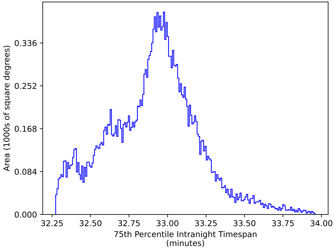
extra_ss_neo3_v3.4_10yrs All sky y band: 75th Percentile Intranight Timespan
