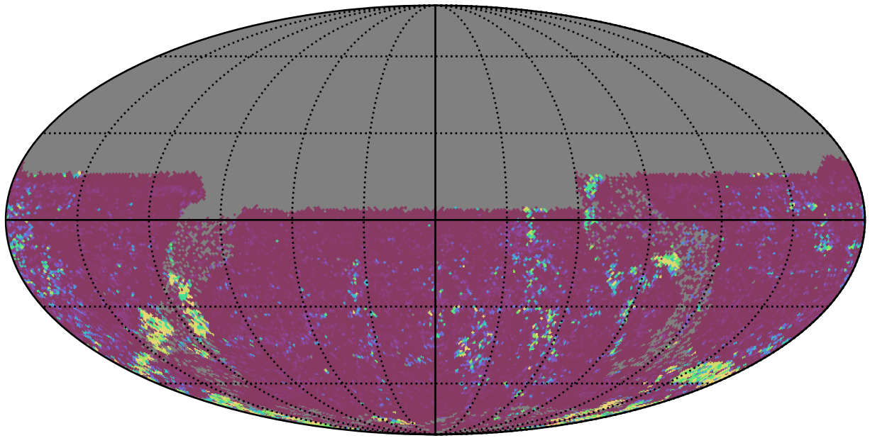
extra_ss_neo3_v3.4_10yrs All sky u band: 75th Percentile Intranight Timespan
