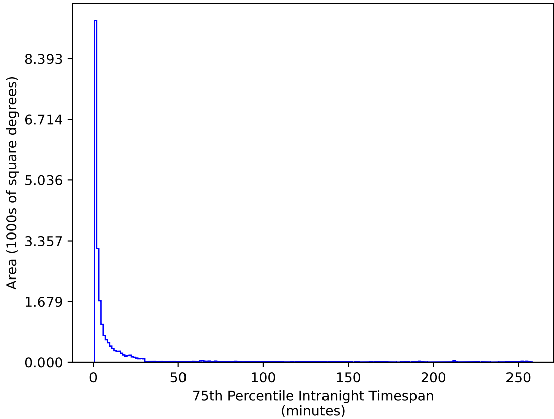
extra_ss_neo3_v3.4_10yrs All sky u band: 75th Percentile Intranight Timespan
