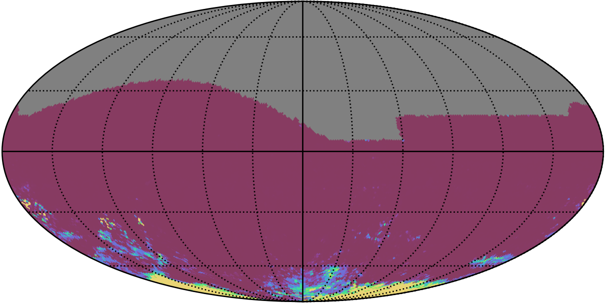
extra_ss_neo3_v3.4_10yrs All sky ri bands: 75th Percentile Intranight Timespan
