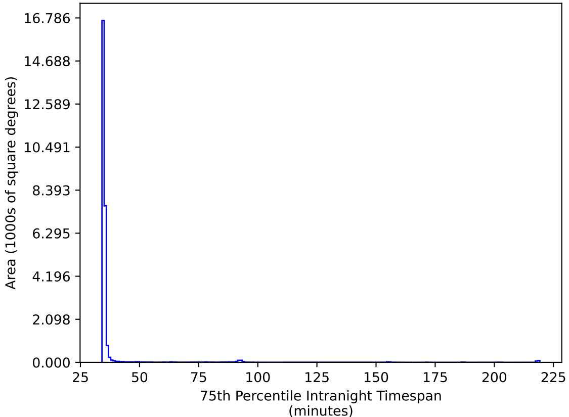
extra_ss_neo3_v3.4_10yrs All sky ri bands: 75th Percentile Intranight Timespan
