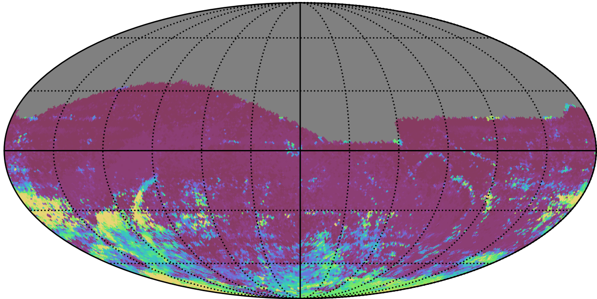
extra_ss_neo3_v3.4_10yrs All sky r band: 75th Percentile Intranight Timespan
