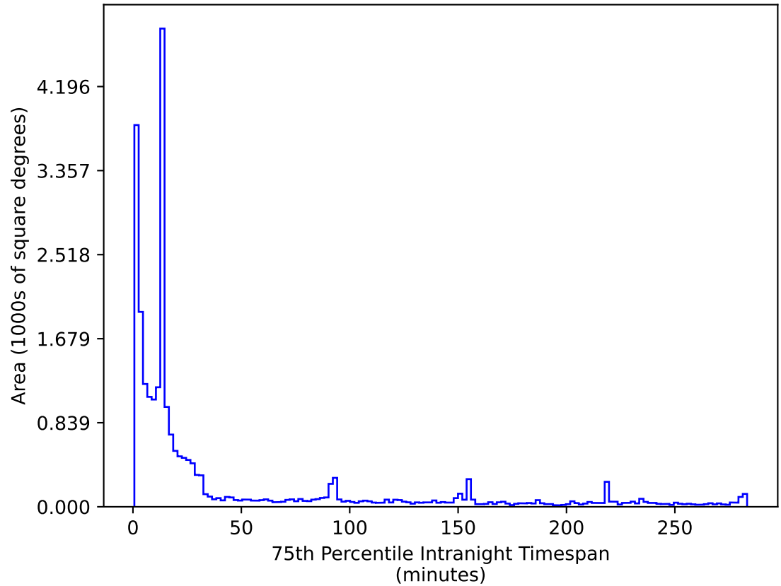
extra_ss_neo3_v3.4_10yrs All sky r band: 75th Percentile Intranight Timespan
