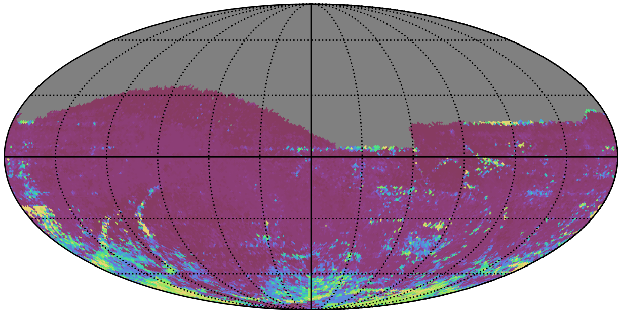
extra_ss_neo3_v3.4_10yrs All sky i band: 75th Percentile Intranight Timespan
