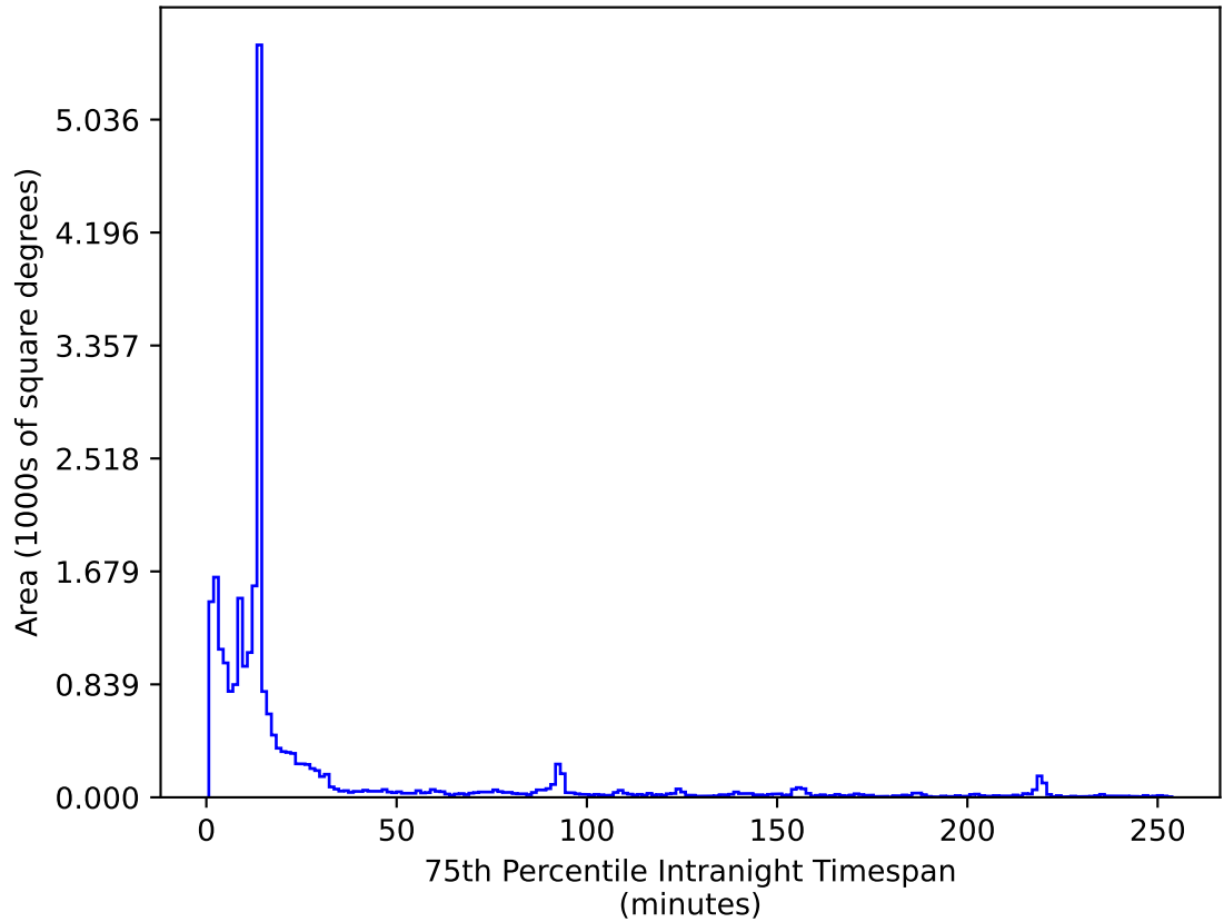
extra_ss_neo3_v3.4_10yrs All sky i band: 75th Percentile Intranight Timespan
