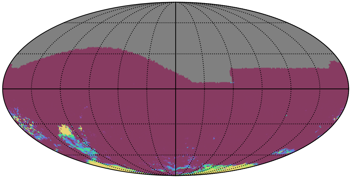
extra_ss_neo3_v3.4_10yrs All sky gr bands: 75th Percentile Intranight Timespan
