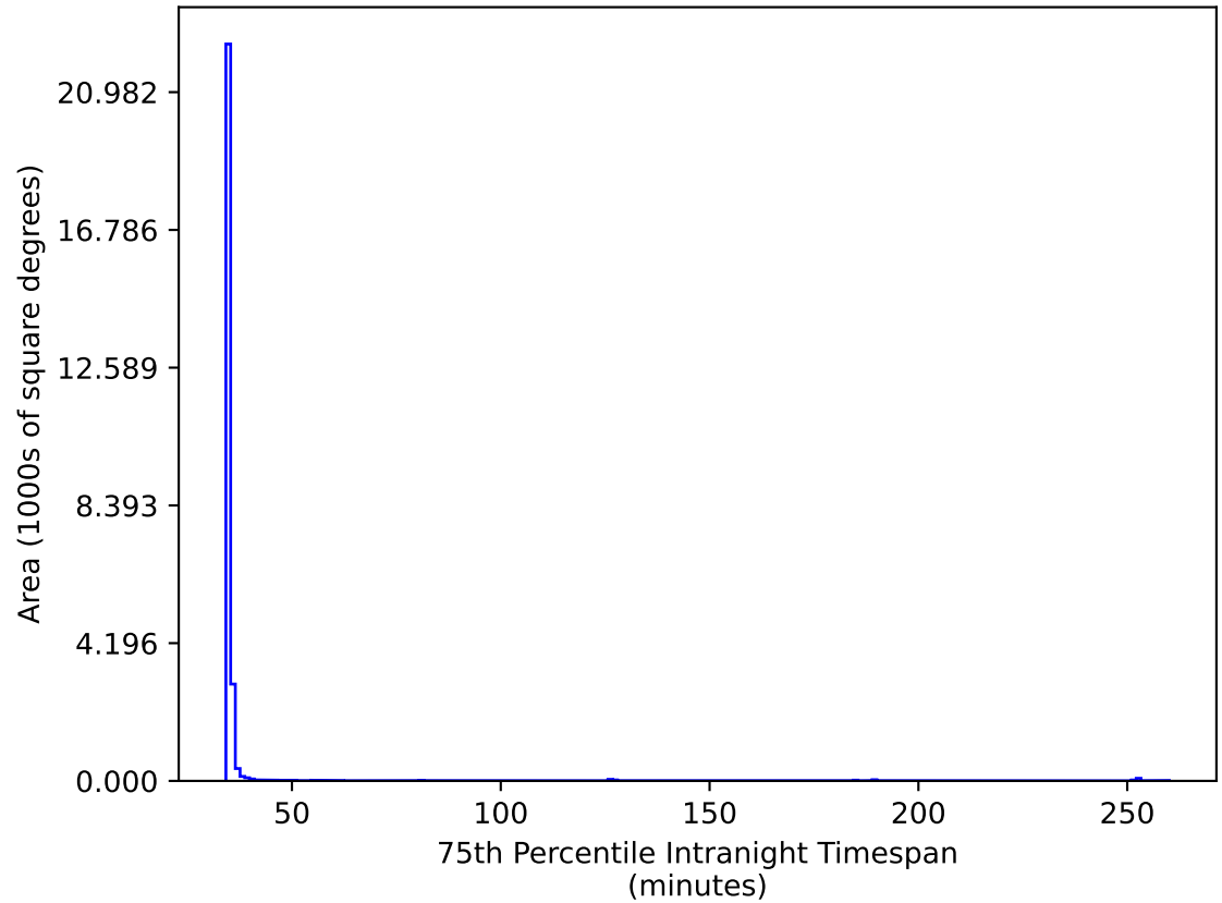
extra_ss_neo3_v3.4_10yrs All sky gr bands: 75th Percentile Intranight Timespan
