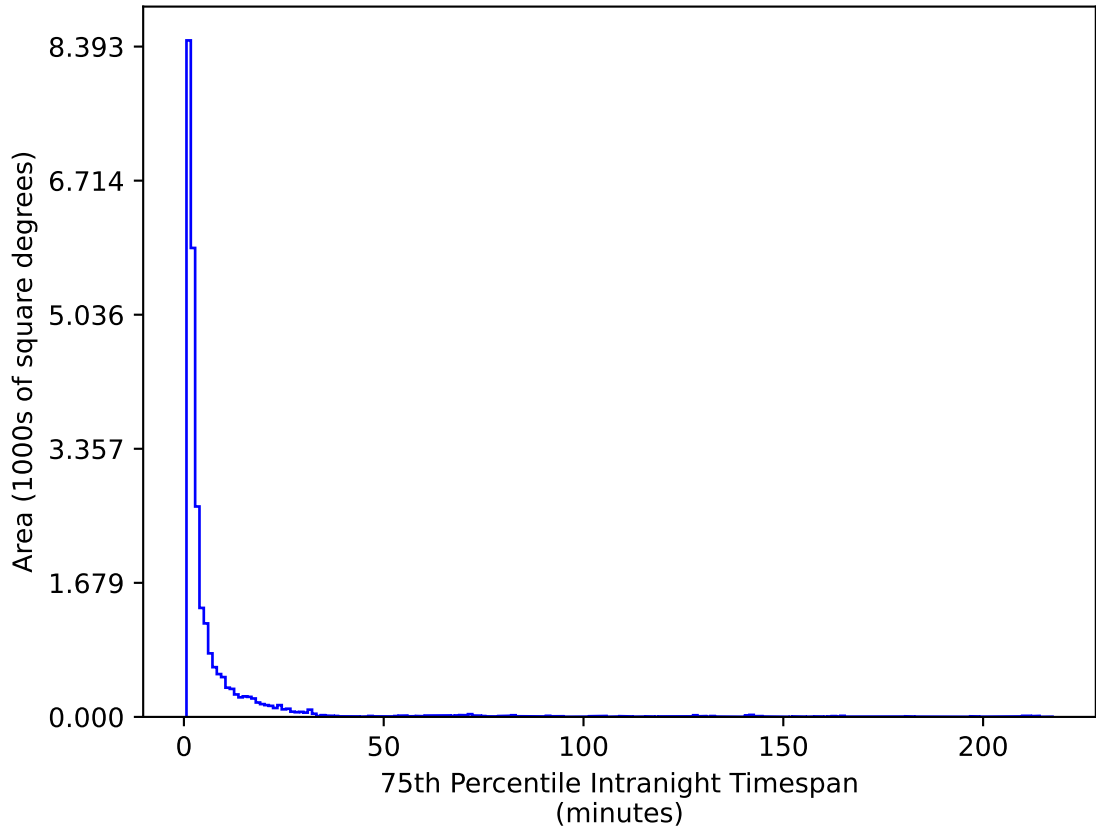
extra_ss_neo3_v3.4_10yrs All sky g band: 75th Percentile Intranight Timespan
