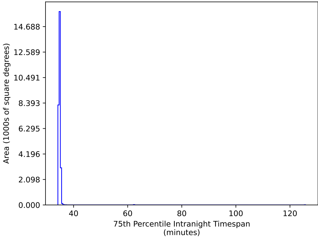
extra_ss_neo3_v3.4_10yrs All sky all bands: 75th Percentile Intranight Timespan
