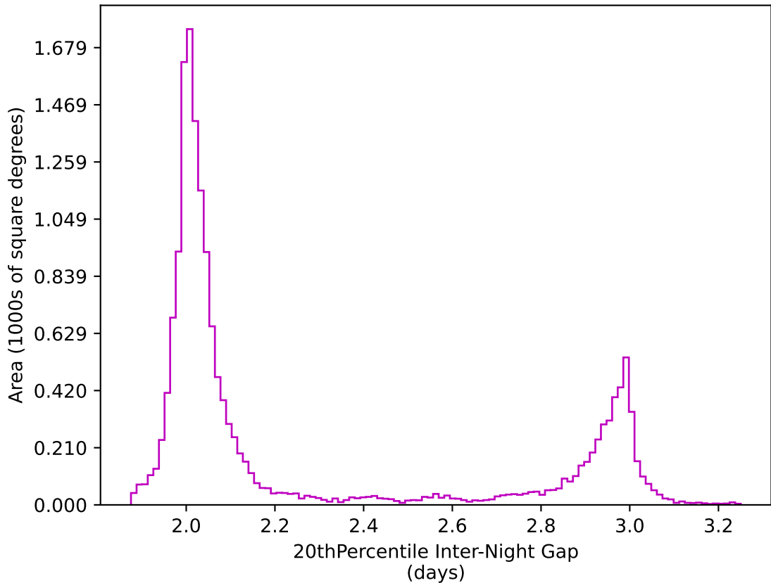
extra_ss_neo3_v3.4_10yrs WFD z band: 20thPercentile Inter-Night Gap
