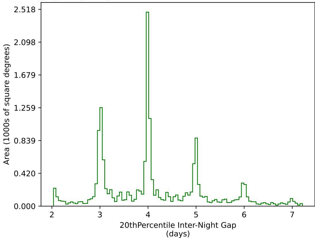
extra_ss_neo3_v3.4_10yrs WFD g band: 20thPercentile Inter-Night Gap
