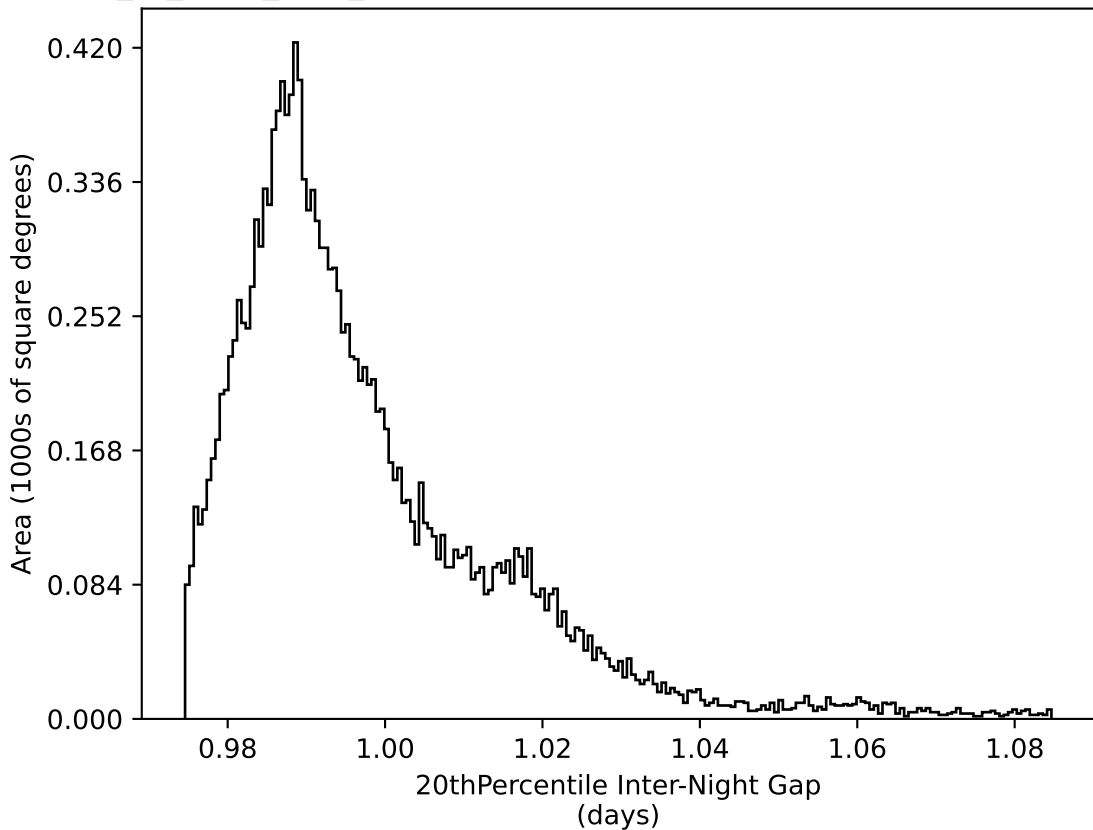
extra_ss_neo3_v3.4_10yrs WFD all bands: 20thPercentile Inter-Night Gap
