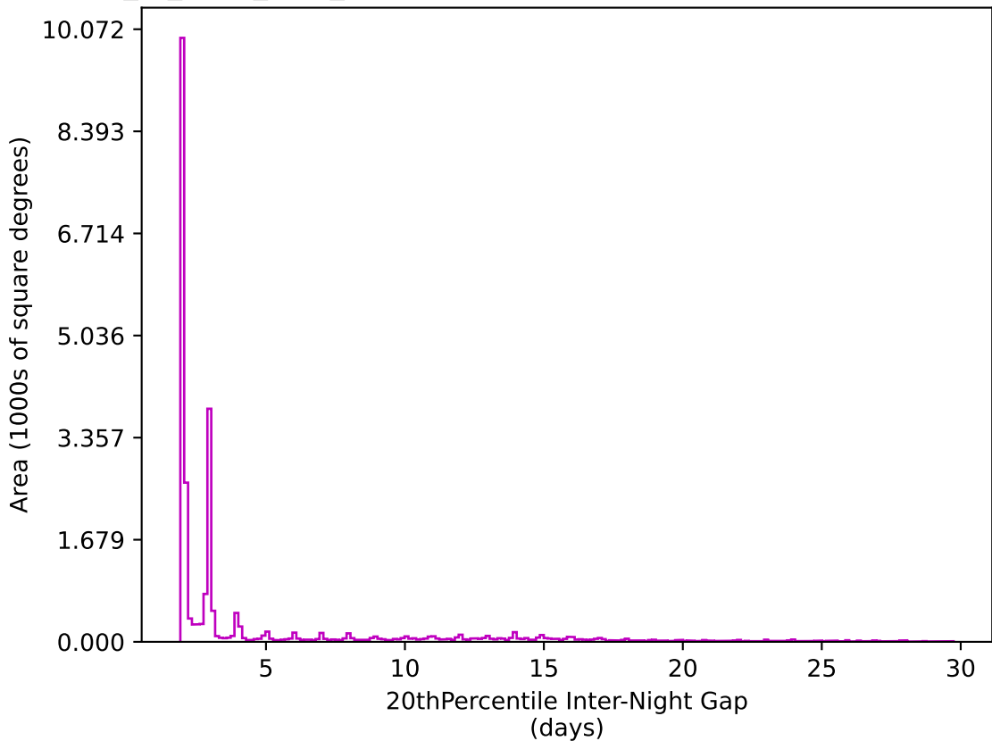
extra_ss_neo3_v3.4_10yrs All sky z band: 20thPercentile Inter-Night Gap
