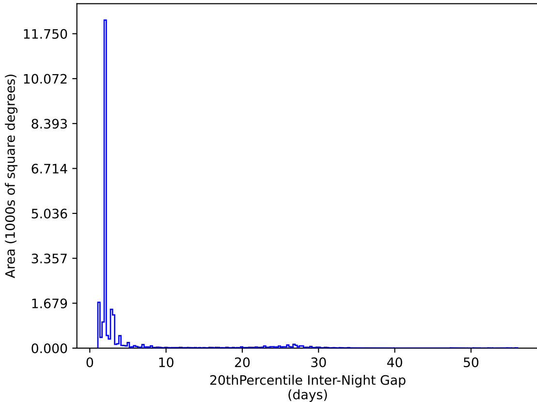
extra_ss_neo3_v3.4_10yrs All sky y band: 20thPercentile Inter-Night Gap
