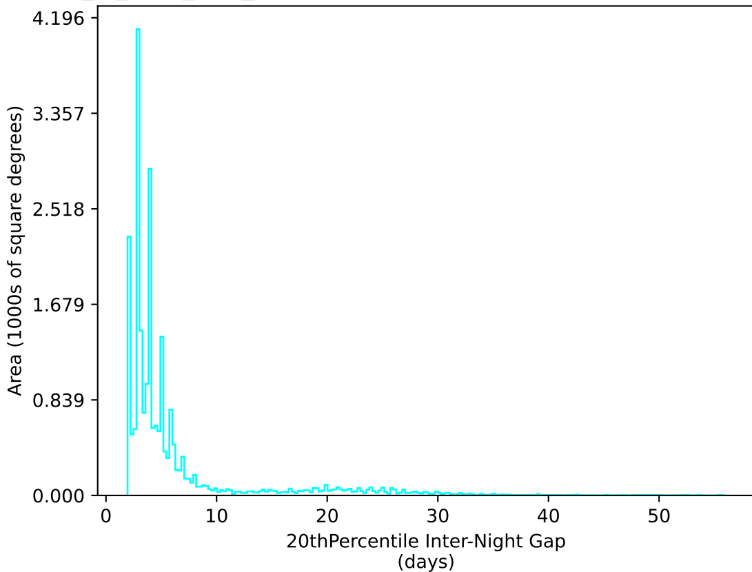
extra_ss_neo3_v3.4_10yrs All sky u band: 20thPercentile Inter-Night Gap
