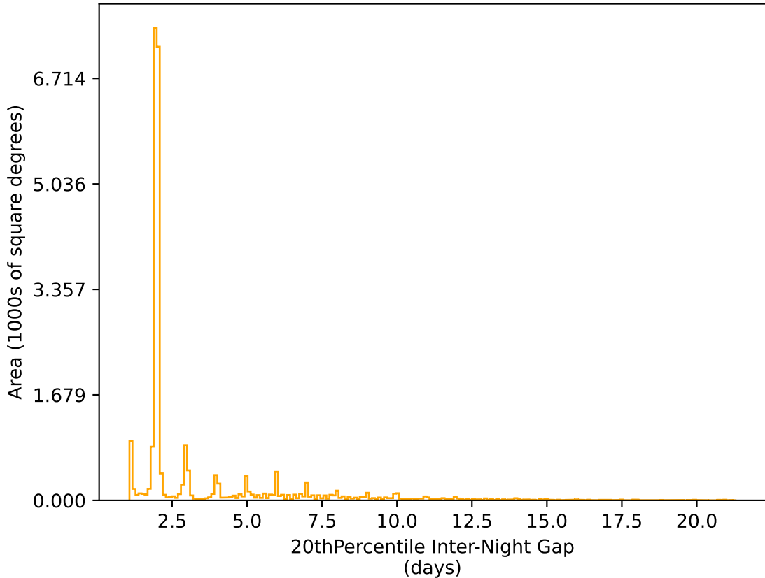
extra_ss_neo3_v3.4_10yrs All sky r band: 20thPercentile Inter-Night Gap
