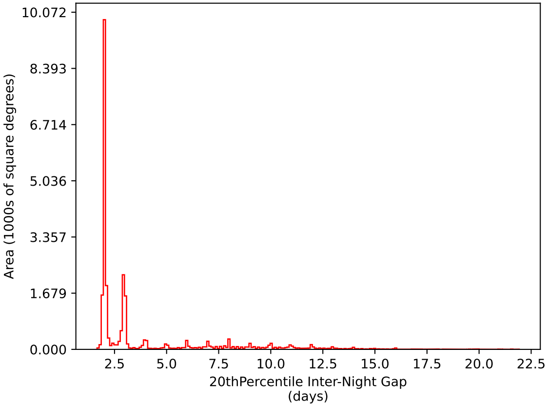
extra_ss_neo3_v3.4_10yrs All sky i band: 20thPercentile Inter-Night Gap
