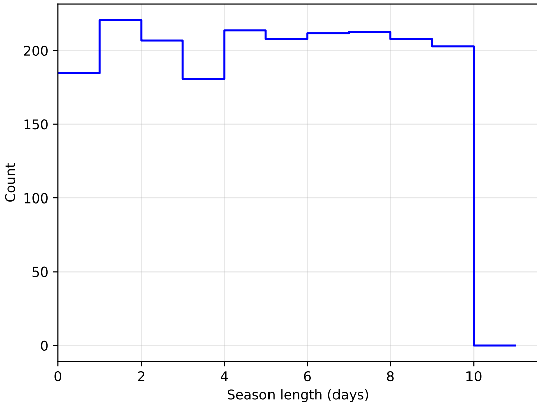
extra_ss_neo3_v3.4_10yrs DD:ELAISS1 all bands: SeasonLength
