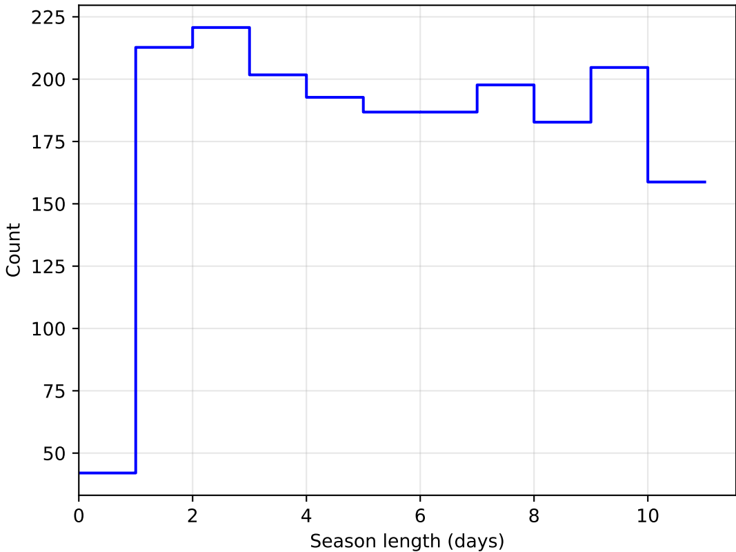
extra_ss_neo3_v3.4_10yrs DD: COSMOS all bands: SeasonLength
