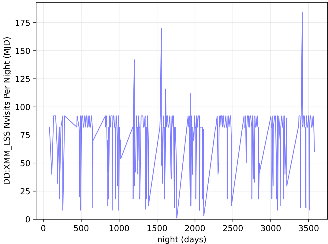
extra_ss_neo3_v3.4_10yrs all bands: DD:XMM_LSS Nvisits Per Night
