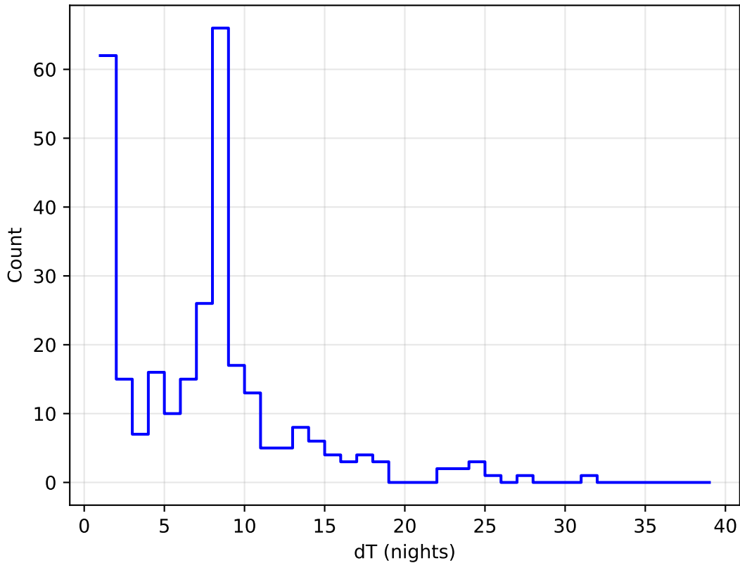
extra_ss_neo3_v3.4_10yrs all bands: DD:XMM_LSS Delta Nights Histogram
