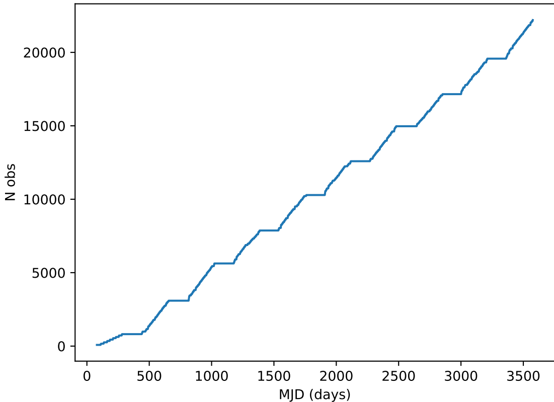
extra_ss_neo3_v3.4_10yrs all bands: DD:XMM_LSS Cumulative NVisits
