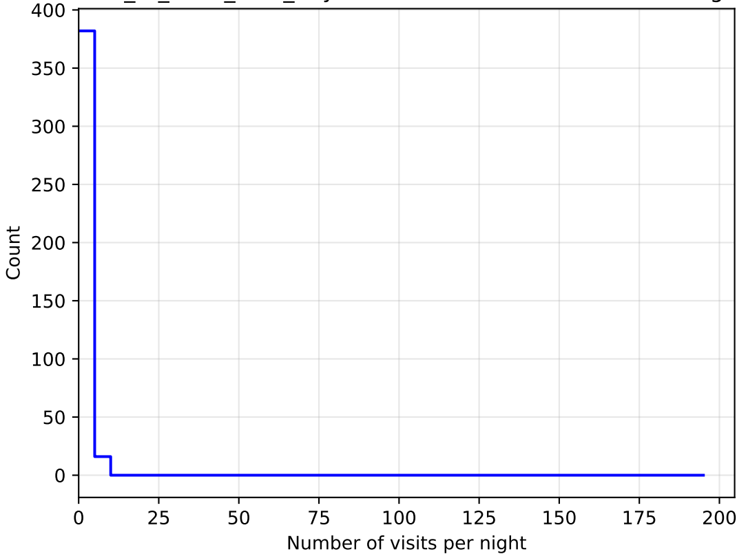
extra_ss_neo3_v3.4_10yrs all bands: DD:WFD NVisitsPerNight
