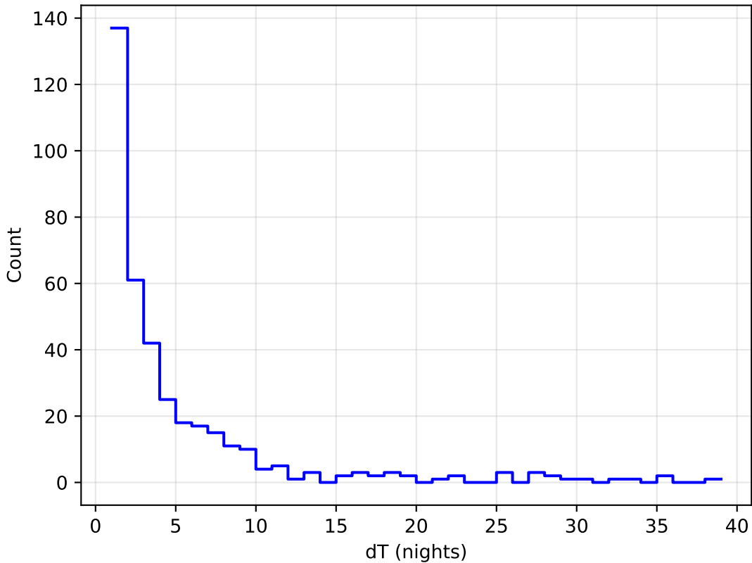
extra_ss_neo3_v3.4_10yrs all bands: DD:WFD Delta Nights Histogram
