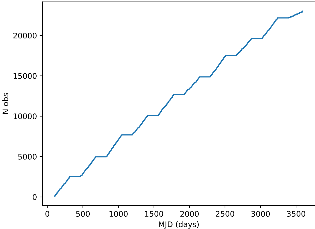
extra_ss_neo3_v3.4_10yrs all bands: DD:EDFS Cumulative NVisits
