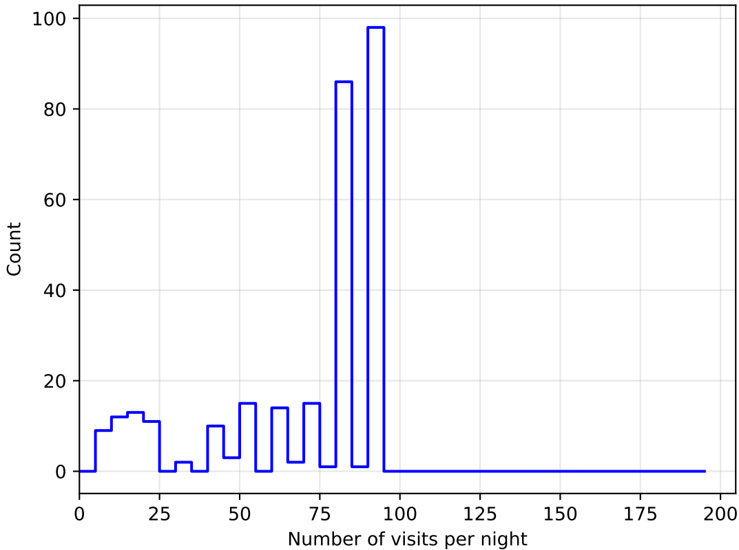
extra_ss_neo3_v3.4_10yrs all bands: DD:ECDFS NVisitsPerNight
