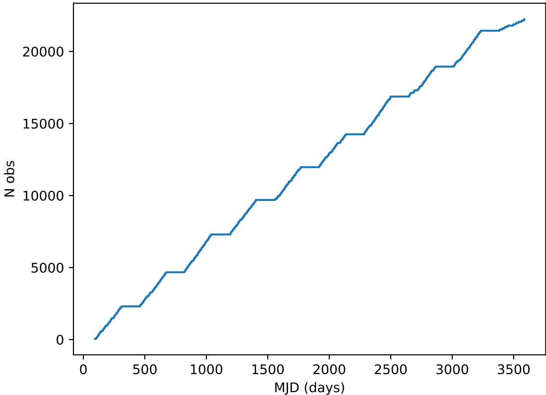
extra_ss_neo3_v3.4_10yrs all bands: DD:ECDFS Cumulative NVisits
