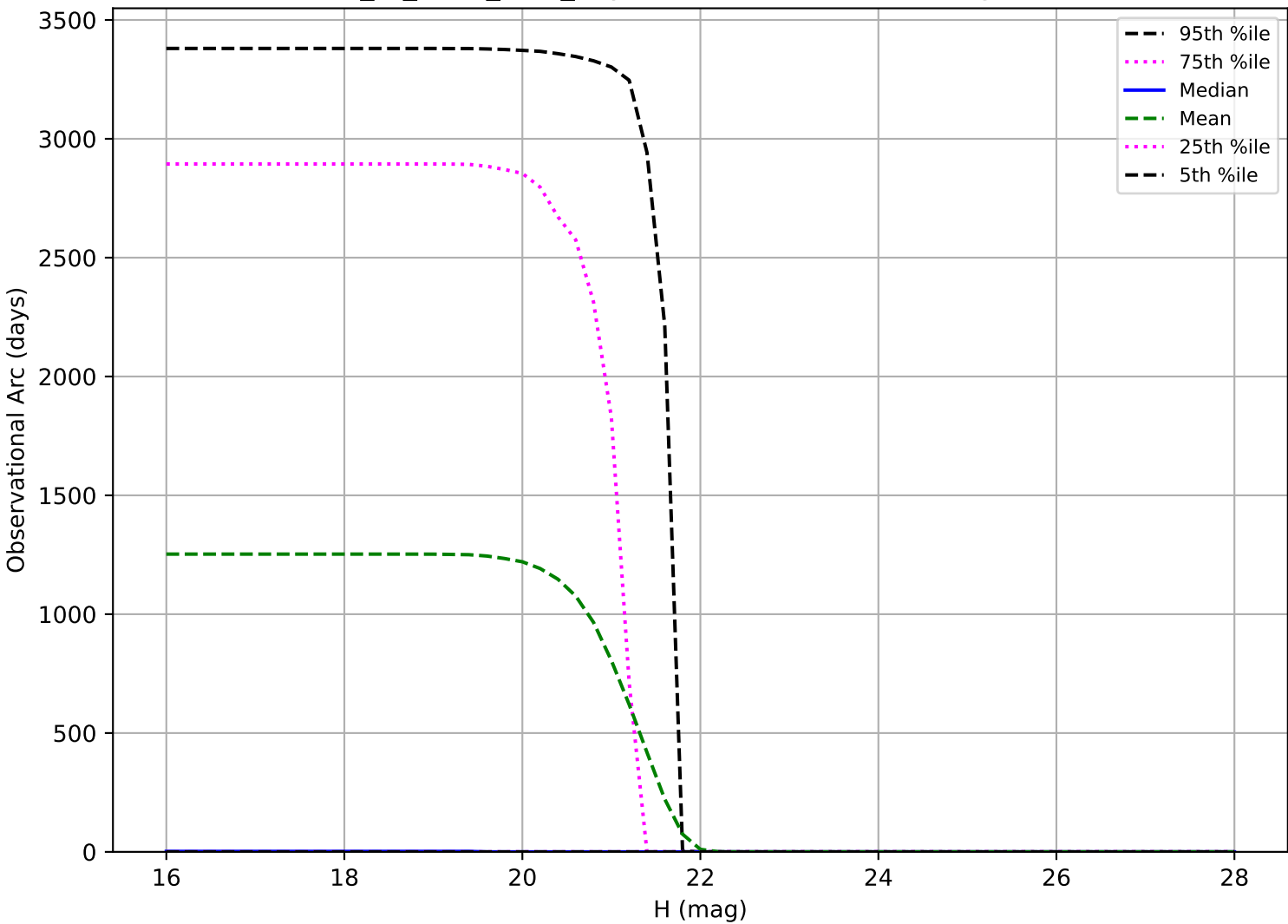
extra_ss_neo2_v3.4_10yrs: Observational Arc Length Vatira
