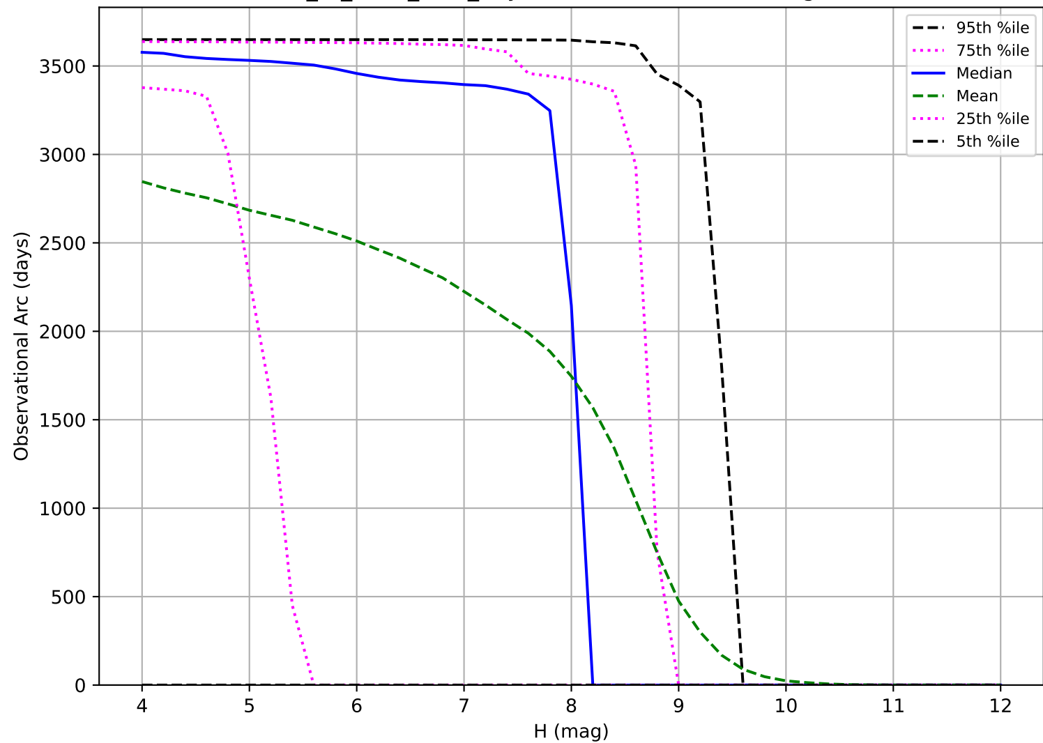
extra_ss_neo2_v3.4_10yrs: Observational Arc Length TNO
