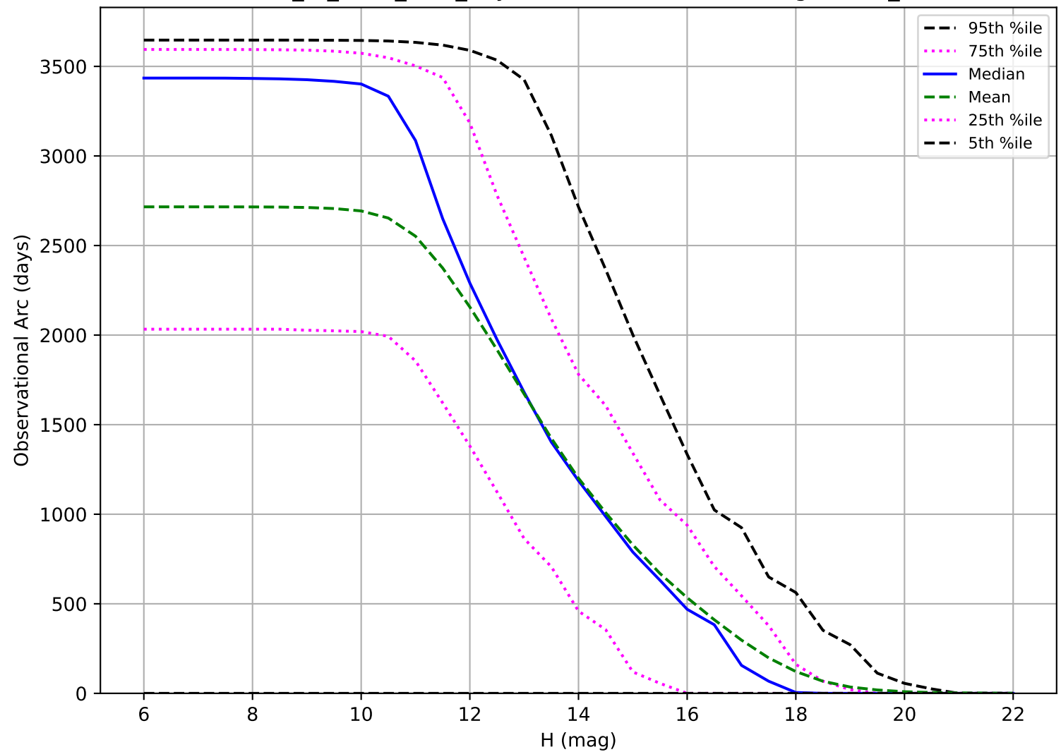
extra_ss_neo2_v3.4_10yrs: Observational Arc Length OCC_r5
