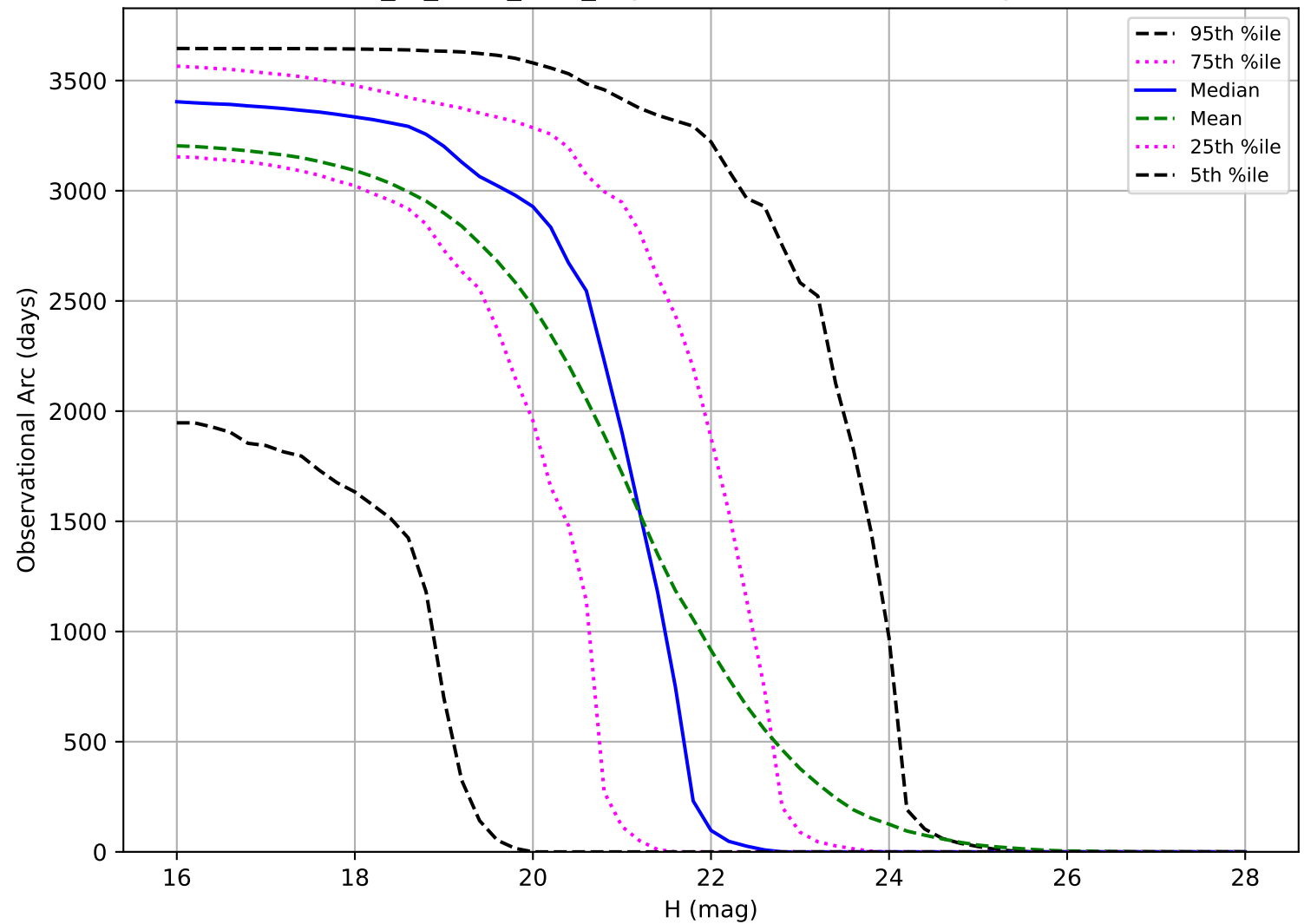
extra_ss_neo2_v3.4_10yrs: Observational Arc Length NEO
