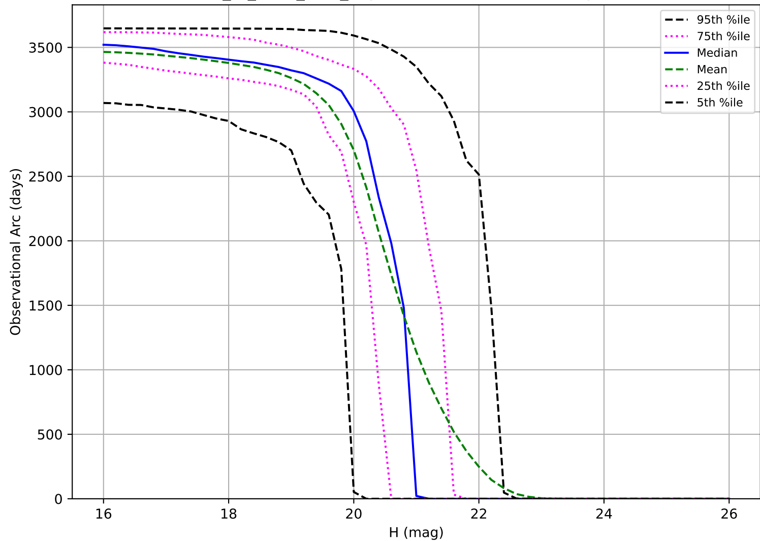
extra_ss_neo2_v3.4_10yrs: Observational Arc Length MBA
