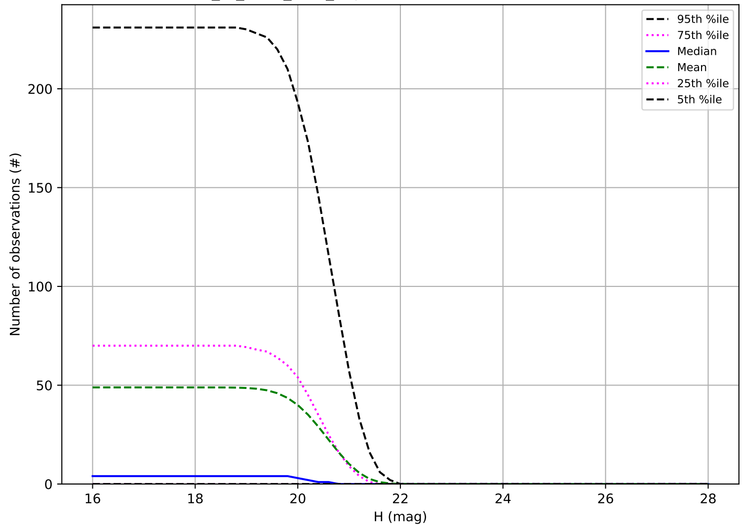
extra_ss_neo2_v3.4_10yrs: Number of observations Vatira
